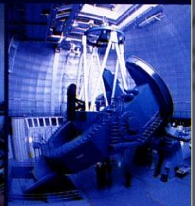
3.5-m Calar Alto Calar Alto, Spain • 1984
