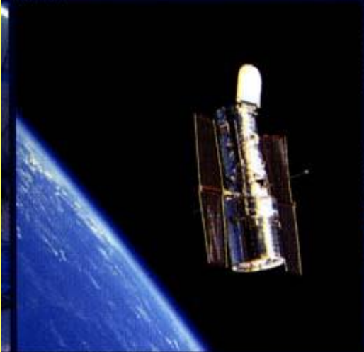
2.4-m Hubble Space Telescope Earth orbit • 1990
