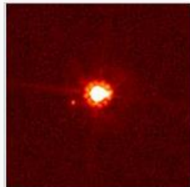
Eris (2005)
