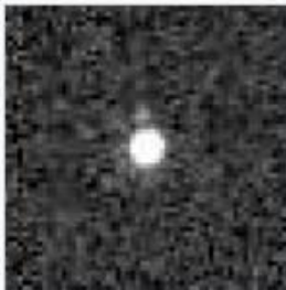
Gonggong (2007)
