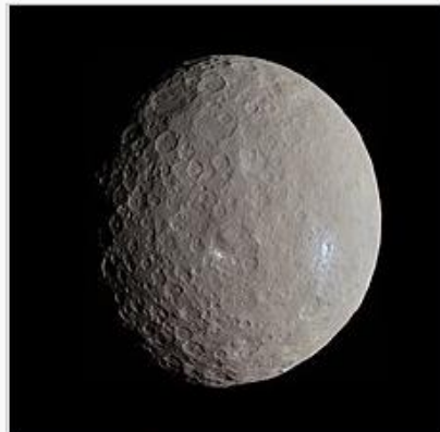
Ceres (1801)
