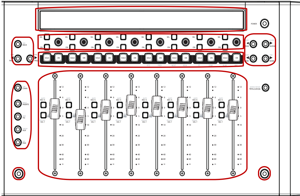
Avid Artist Mix: Display, Knob Set navigation, Sel/On keys and touch-sensitive knobs, Solo/On keys, Fader navigation, Knob Set selections, Fader strips, Shift key, Shift key
