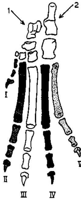
LUPUS post.
