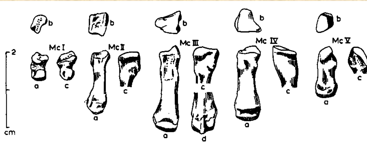
CASTOR
