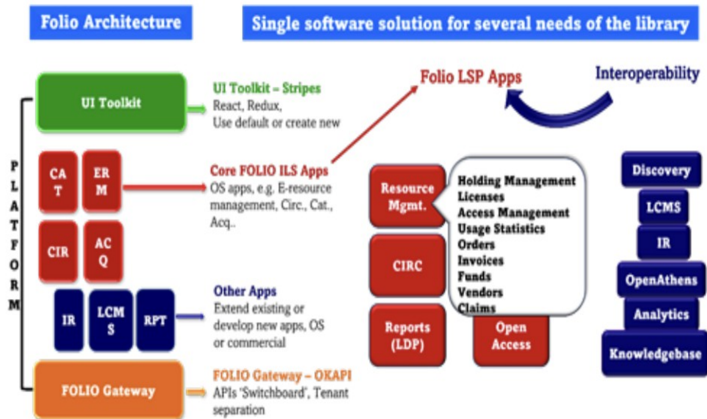
Figure 4. FOLIO architecture.
