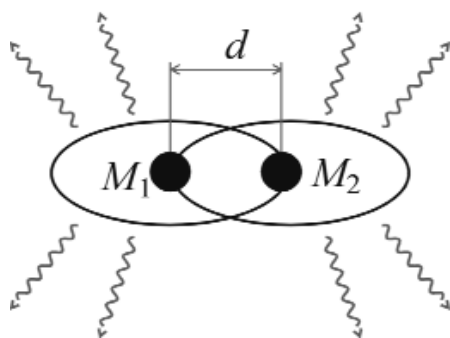
PSR 1913+16
