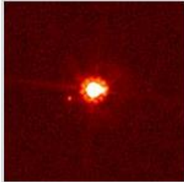
Eris (2005)
