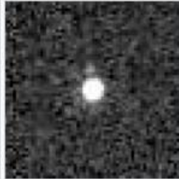
Gonggong (2007)
