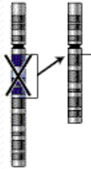
Deletion
