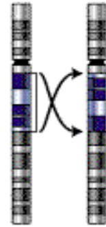
Inversion
