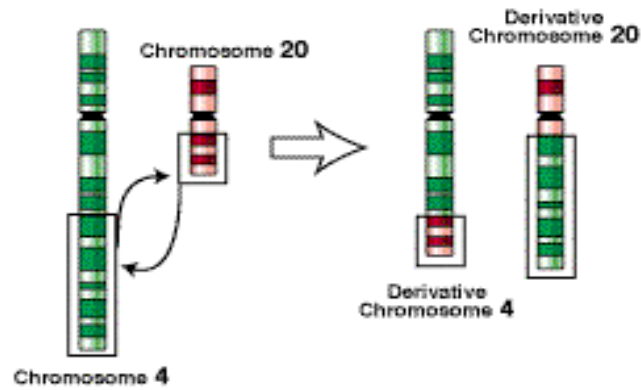
Translocation
