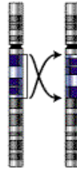
Inversion
