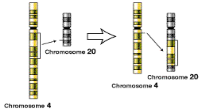
Translocation
