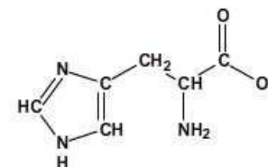
histidin (His)
