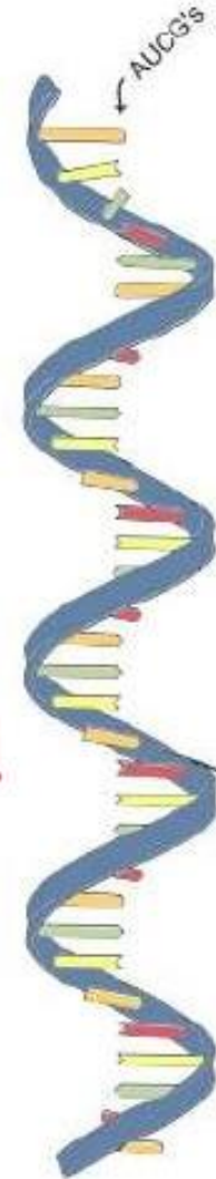
RNA
