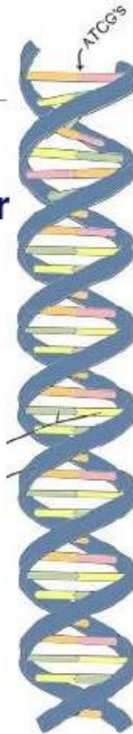
DNA
