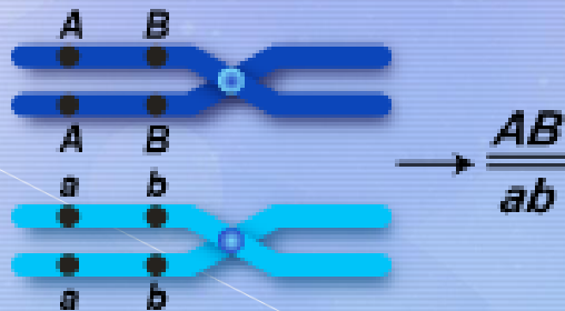
CIS konfigurace (coupling)
