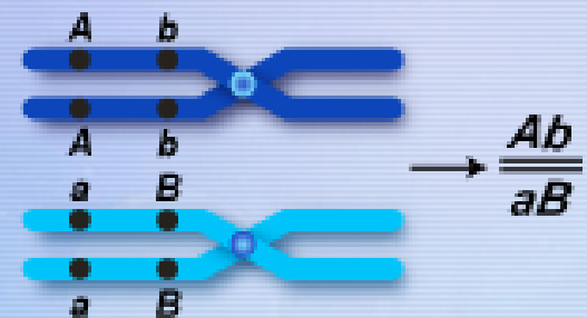
TRANS konfigurace (repulsion)
