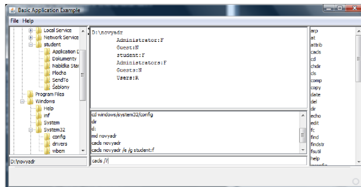
Fig. 1. Simple Application for Windows Administration Training
